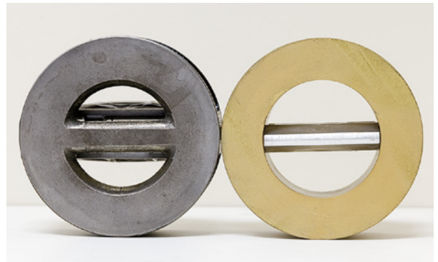
Our elastomer hinge design (on right) eliminates the check valve seat, provides greater open area and lower pressure drop compared to traditional metal hinge dual plate wafer check valves.
